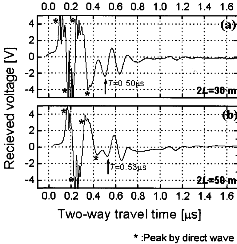
Fig. 9. The time series of radio echo at High Camp. a: Antenna separation was 30 m; b: Antenna separation was 50 m. Arrows indicate clear reflections that we interpreted the echo from the nadir bedrock beneath the ice.
