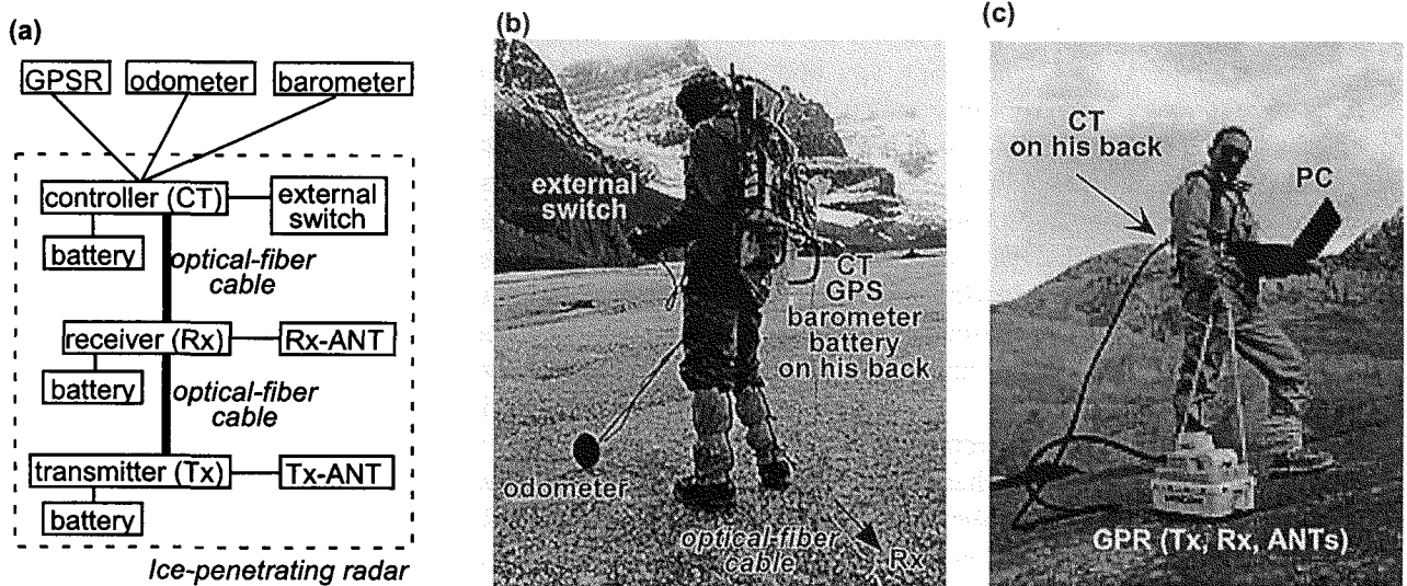
Fig. 3. Tested instruments. (a) Block diagram of the glacier profiler system. Thick and thin lines show optical-fiber and electrical cables, respectively. Length of electrical cables is less than 2 m. Antennas (ANTs) are directly connected to the Tx and Rx. (b) Photo of the glacier profiler system. Although there are both external switch and odometer, each of them can be used for the triggering at a time. (c) Photo of the ground-penetrating radar (GPR). Package on the glacier contains antennas, Rx and Tx. The CT triggers Tx and Rx according to given observation parameters from the PC. Also, the PC displays quick-look data.
