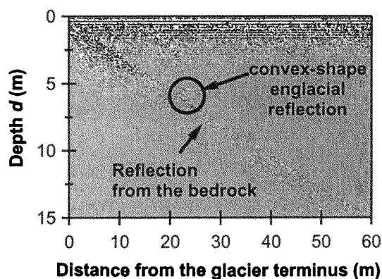
Fig. 5. Pseudo-cross section of the glacier terminus obtained with GPR. Stronger and smaller received signals represent with darker and lighter colors. A continuous echo between the left top and the right bottom is from the subglacial interface. The circle shows the location of a convex-shape englacial reflection.
