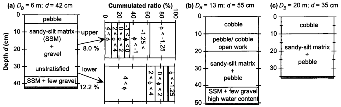
Fig. 2. Debris stratigraphy at (a) D_B = 6 m, (b) D_B = 13 m, and (c) D_B = 20 m along the line B. The depth ( d ) at each site is given at the top of each panel. Gray bands represent top surfaces of the core ice. Sites (a) and (b) are on the top flat area of the lateral moraine, whereas the site (c) is on the steep slope. SSM represents sandy-silt matrix. Note that water contents and grain-size distribution represent with weight percent and phai scale, respectively.
