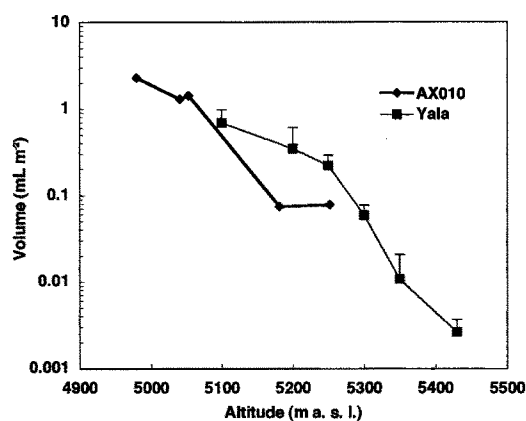
Fig. 5. Altitudinal change of algal biomass (mL m -2 ) estimated by measuring the total algal volume.
