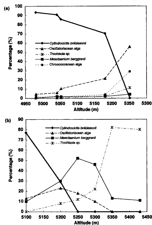
Fig. 6. Altitudinal change of community structure which was represented by the proportion of each algae to the total algal biomass (a) AX010 (b) Yala glacier (modified after Yoshimura et al. , 1997).
