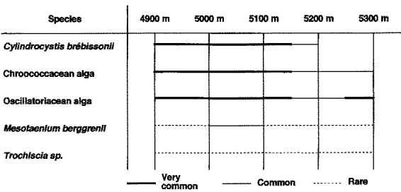
Fig. 4. Algal distribution range and relative frequency of occurrence on the glacier.
