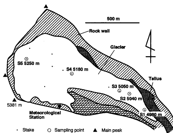
Fig. 2. A map of Glacier AX010 showing the locations of sampling points on the glacier October 1995. Dots show the locations of the stakes for mass balance study.
